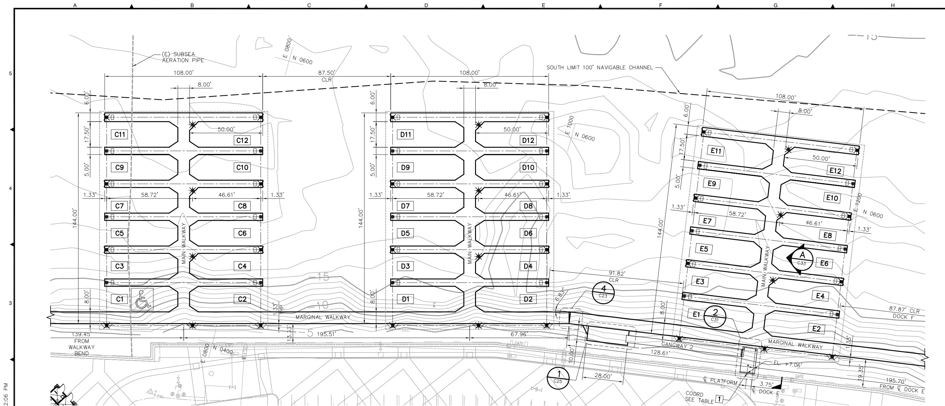
C PLAN - DOCK C SCALE: 1"=20'
